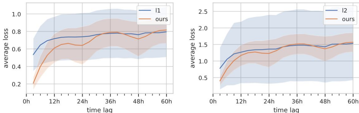
Figure 4: Mean l_1 -norm (left) and mean l_2 -norm (right) between samples that are a fixed time-interval apart, calculated on the training set. Shaded areas indicate standard deviation. For comparability, the AtmoDist distance has been normalized in each case with the method described in Appendix A.3 . To give equal weight to divergence and vorticity, they have been normalized to zero mean and unit variance before calculating pixel-wise metrics.
