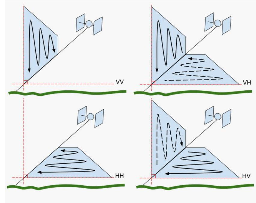
Figure 2: SAR signals are transmitted and received either vertically (V) or horizontally (H). This gives the potential for four different polarization combinations (transmit listed first, receive second): VV, VH, HH, and HV. Credit: ASF
